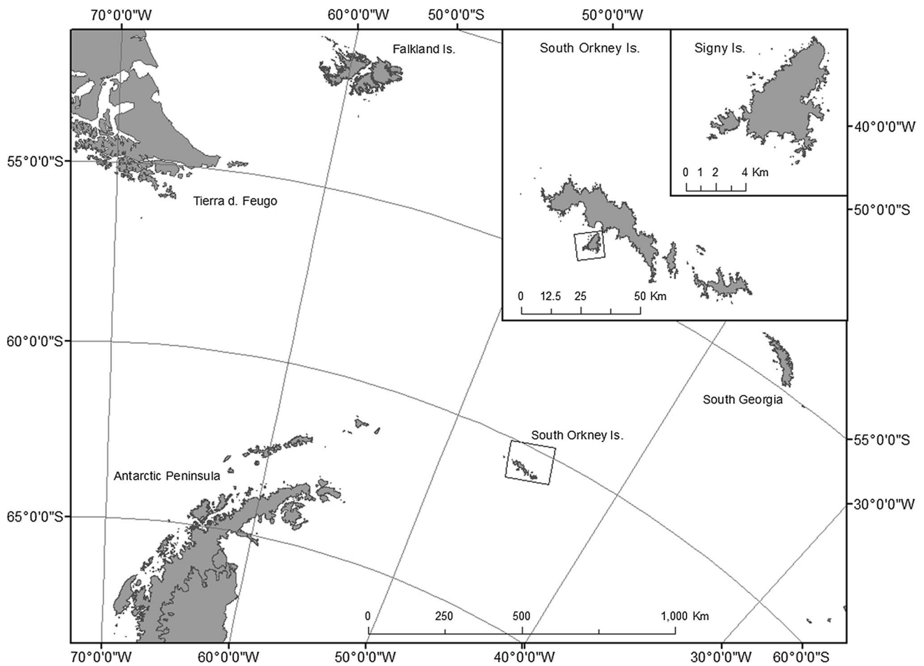
Fig. 1 Maps showing the Location of the South Orkney Islands and Signy Island in the Southern Ocean. Inset—Map of Signy Island, with Research Station (and thus current area of E. murphyi distribu-
