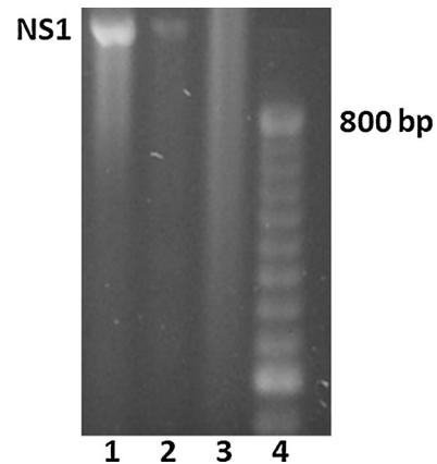
Fig. 1B Construction of recombinant Agrobacterium tumefaciens lineage for expression of dengue virus-2 NS1 gene. b Amplification of NS1 gene in Agrobacterium tumefaciens transformed with pCAMBIA 3301/NS1 plasmid. 1 and 2 representative samples of transformed A. tumefaciens ; 3 negative control (representative untransformed A. tumefaciens ); 4 100 bp DNA marker
