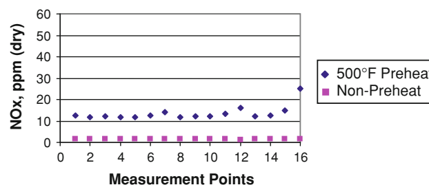
Fig. 9 NO x Measurements in RQL fuel-rich zone ( x/R = -1 ) for preheat and non-preheat conditions
