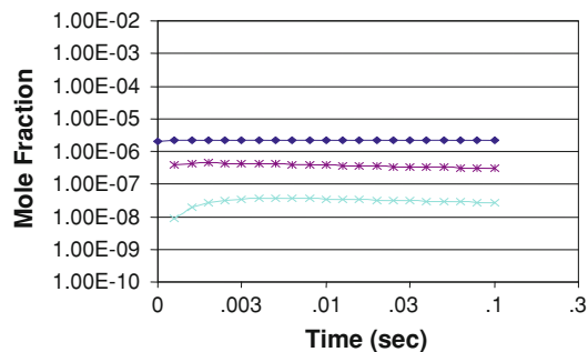
(c) Temp = 1350K, \phi = 0.45
