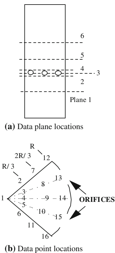
Fig. 5 Measurement locations
