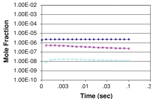
(b) Temperature = 1450 K, \phi = 0.45
