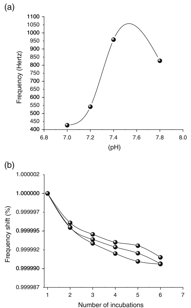
Fig. 6 Immunosenor response as function of pH (a) and reproducibility of the immunosenor from three different electrodes response (b)
