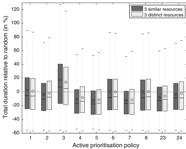
Fig. 11 Comparison of policy performance for the chainsaw product model. Simulations were run with (1) three identical resources that can work on all components and (2) three different resources that can only work on specific components
