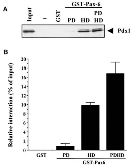
Fig. 6A, B. Pdx1 interacts with the HD of Pax-6. (A) GST-precipitation assay using 10 \mu g of GST alone, GST-Pax-6 paired (PD), homeo (HD) or paired-linker-homeodomain (PDHD), fusion proteins immobilized on sepharose beads and in vitro synthesized, 35 S-labelled Pdx1. Lane input, 10% of the respective in vitro translation reaction used for protein to protein interaction. (B) Quantification of protein interactions shown in (A) as the precipitation rates relative to the respective input. Data are presented as the mean \pm SEM of at least three experiments
