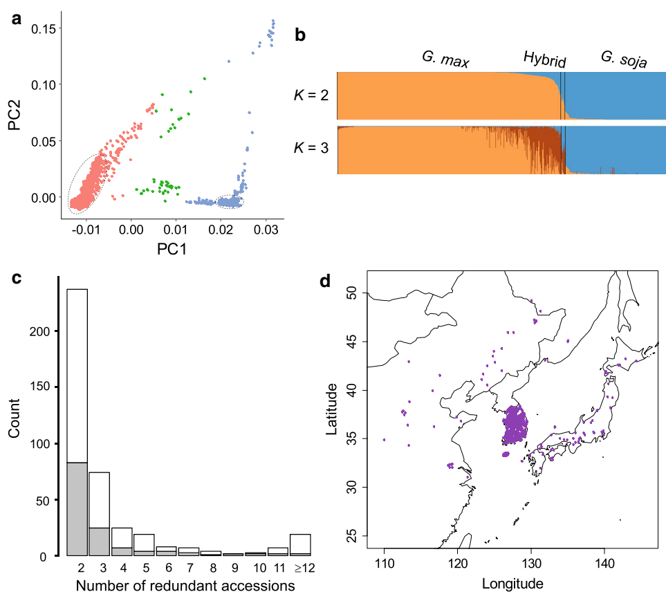
Fig. 1 Population structure of the genotyped 4234 soybean accessions. a Principal components of SNP variation. PC1 and PC2 indicate score of principal components 1 and 2, respectively. Each of PC1 and PC2 explained 15.6% and 2.7% of variance in the data. Glycine max , G. soja , and hybrids are shown by red, blue, and green dots, respectively. The majority of Korean accessions cluster together within dashed ellipses. b ADMIXTURE plots. The accessions were divided into three groups: G. max , G. soja , and their hybrids. c Distribution of number of redundant accession groups that showed < 1.25% inconsistencies between the SNP calls. G. max and G. soja are shown by white and gray boxes. d Geographic distribution of the collection sites for G. soja accessions
