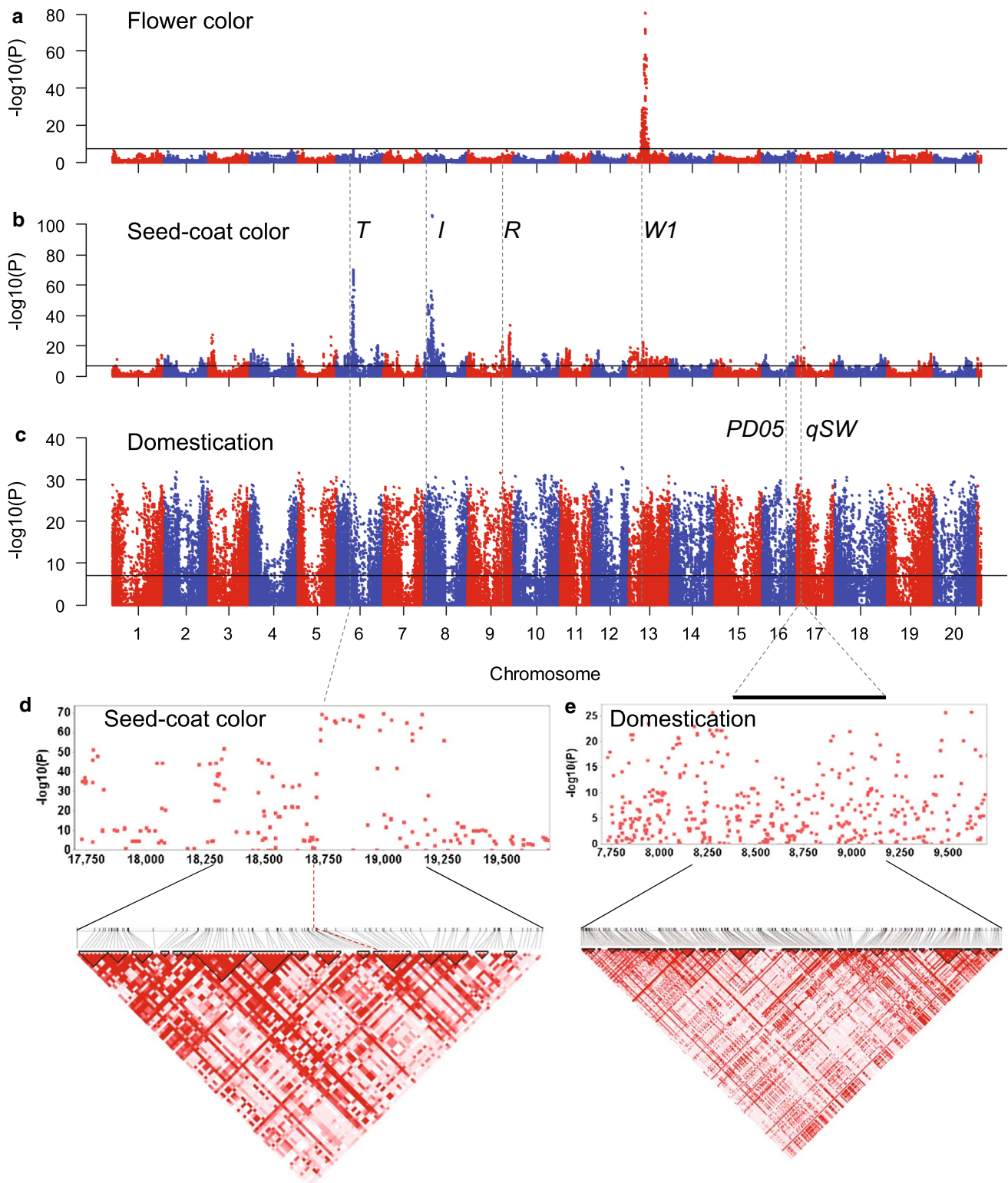
Fig. 3 Genome-wide association scans for 3036 soybean accessions for flower color, seed-coat color, and domestication. a Manhattan plot for flower color. The solid horizontal line denotes the Bonferroni-adjusted significance threshold. Chromosomal regions of known genes ( T , I , R , W1 ) or loci ( PD05 and qSW ) are indicated by dashed vertical lines. b Manhattan plot for seed-coat color. c Manhattan plot
