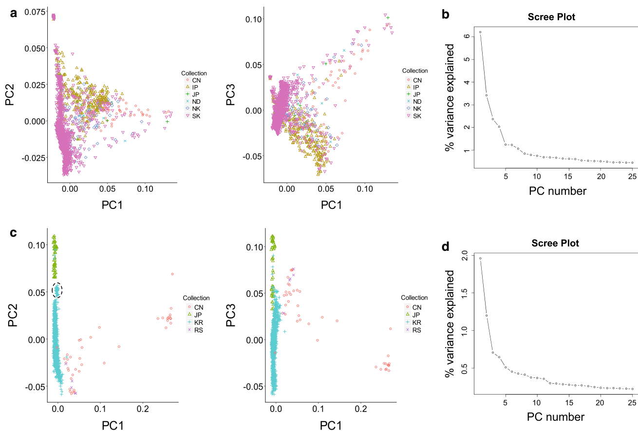
Fig. 2 Population structures of 1957 domesticated and 1079 wild soybean accessions in the 3036 non-redundant soybean accession set. a Principal components (PC) of SNP variation in the domesticated population. The plots show the first three principal components. The countries of collection or improvement status of the soybean accessions in a and c are represented by two-letter codes—CN, China; IP, improved breeding line; JP, Japan; ND, not determined; NK, North Korea; RS, Russia; and SK (KR), South Korea. b Scree plot of the
