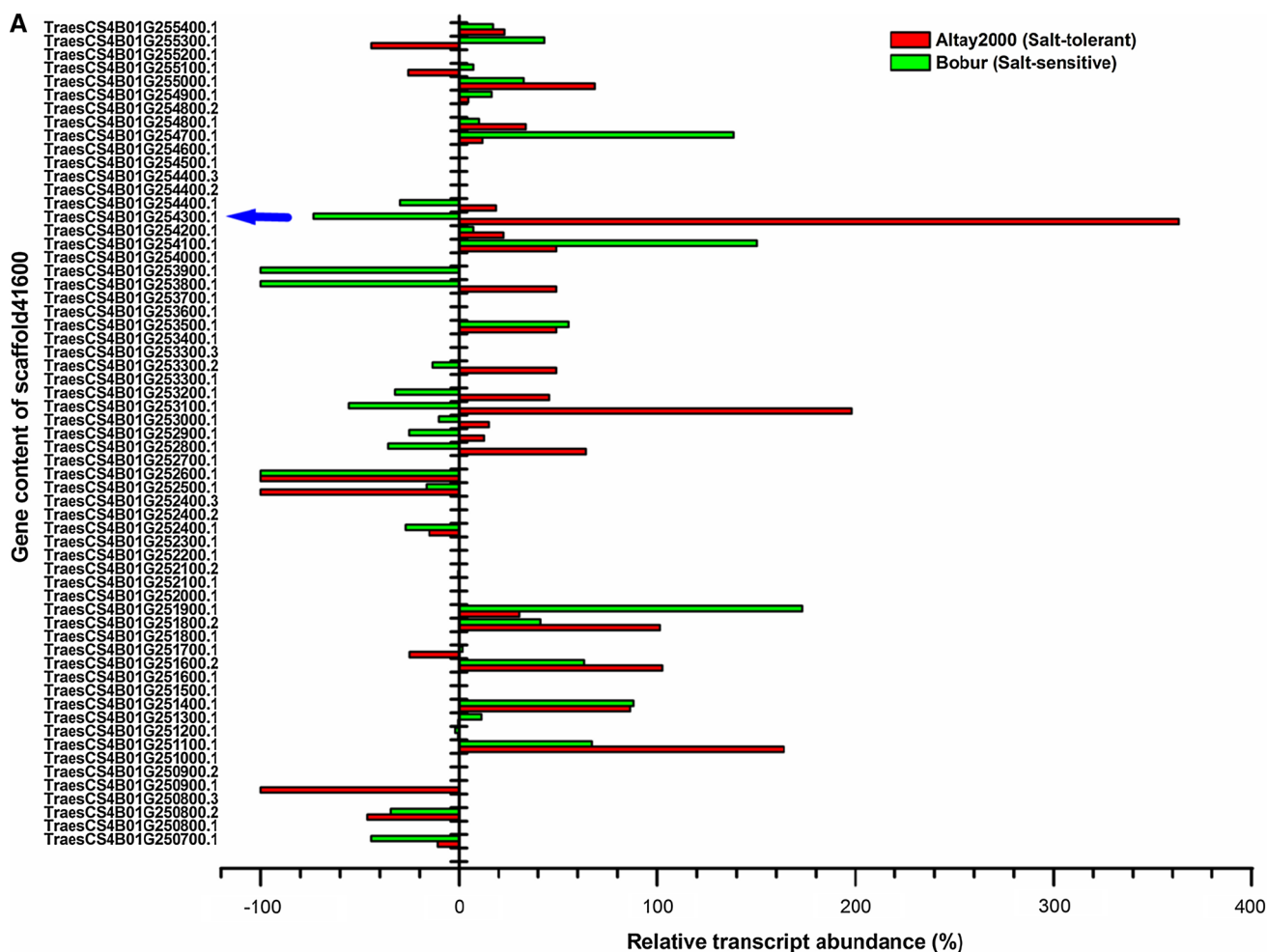
Fig. 5 Relative expression levels of all the annotated genes (in their natural order) belonging to scaffold41600 (~13 Mb) due to salt stress in Altay2000 (salt-tolerant) and Bobur (salt-sensitive) genotypes after 24 days. The relative abundance of the genes was determined as a
