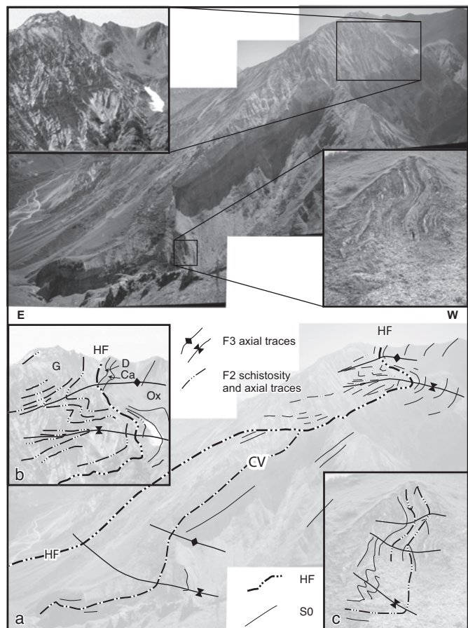
Fig. 6. a) Panoramic view of the D2 Houiller Frontal (HF) thrust and the D1 Cicatrice of Varlossière (CV) east of Cime Noire (Point 2626, bottom of Fig. 7), folded by F3 open folds with gently SW-dipping axial planes. b) F3 folds in gypsum, defining the position of the HF (light rock resting above the line marking the HF in the picture). c) F3 folds in Oxfordian sediments of the SBU below the HF. Ox: Oxfordian schists and breccias Ca: Cancellophycus Formation, D: basal Dogger, G: gypsum. For the explanation of tectonic letter symbols see Fig. 1.
