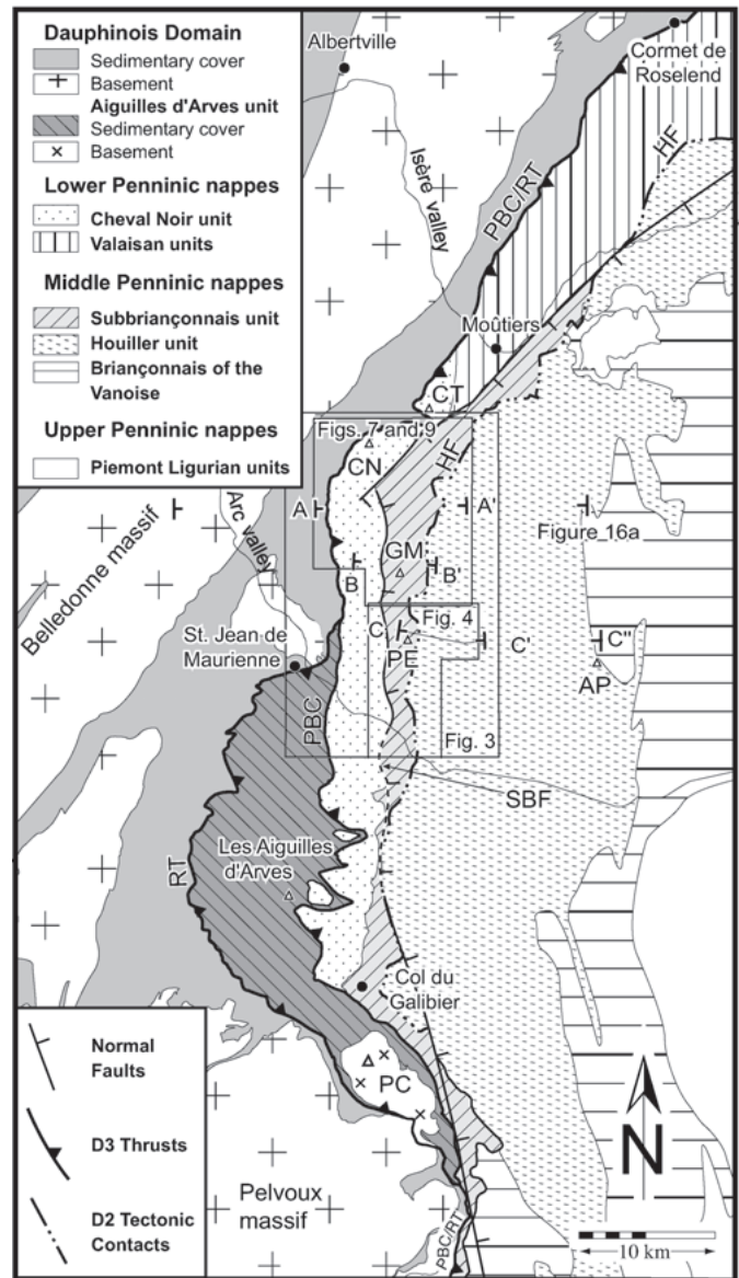
Fig. 1. Tectonic map of the Western Alps between Cormet de Roselend and Pelvoux Massif. Boxes indicate areas covered by Figs. 3, 4, 7 and 9. HF: Houillier frontal thrust; PBC: Penninic Basal contact; RT: Roselend thrust; SBF: Subbriançonnais front (mostly overprinted by normal faulting); AP: Aiguille de Pécelet; GM: Aiguilles de la Grande Moendaz; PC: Pics de Combeynot; PE: Grand Perron des Encombres.
