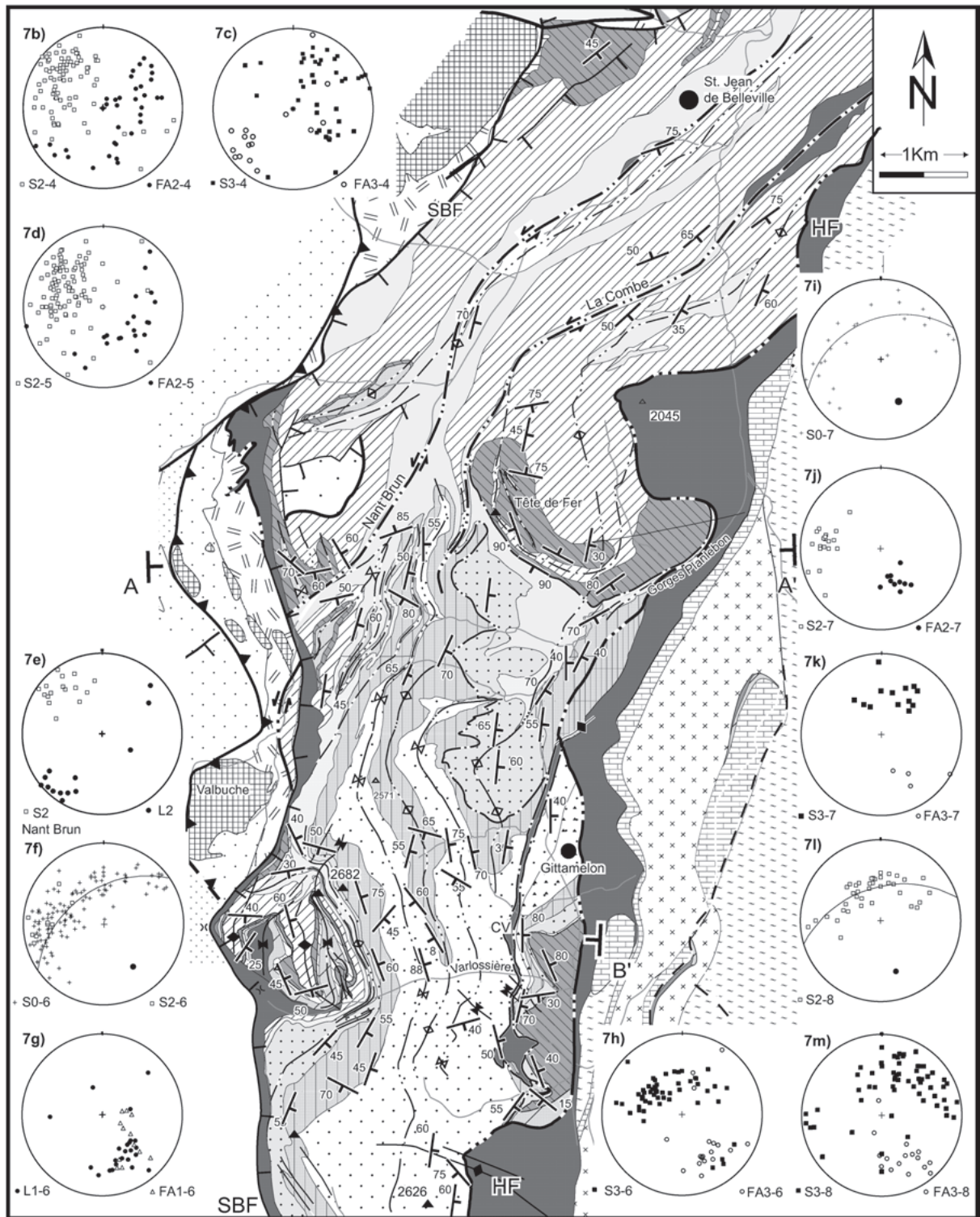
Fig. 7. a) Geological Map of the northern and central part of the Subbriannonnais Unit (SBU) (see Fig. 1 for location). CV: Cicatrice de Varlossière; HF: Houiller Front; SBF: Subbriannonnais Front. For patterns and symbols see legend in Fig. 4b. b) to m): Equal area, lower hemisphere stereoplots. The first symbol besides the stereoplots (e.g. S2 in Fig. 7b) indicates: S0 (=bedding); S2 and S3 schistosités; L1 and L2 stretching lineations; FA2 and FA3 fold axes. The second symbol (e.g. 4 in Fig. 7b) indicates tectonic contacts (Nant Brun) or sub-areas (1, 2 etc.) where the data are from. See Fig. 3 for location of sub-areas. f), i) and l): best fit poles for FA3, determined from folded S0 beddings (f & i) and from folded S2 schistosités (l).
