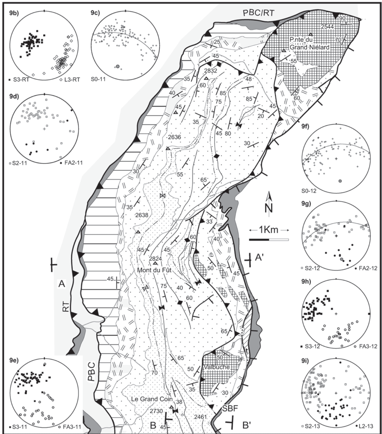
Fig. 9. Geological Map of the Cheval Noir Unit (CNU) between Niéard (north) and Le Grand Coin (south), see Fig. 1 for location, and for tectonic letter symbols. See legend given in Fig. 4b.
