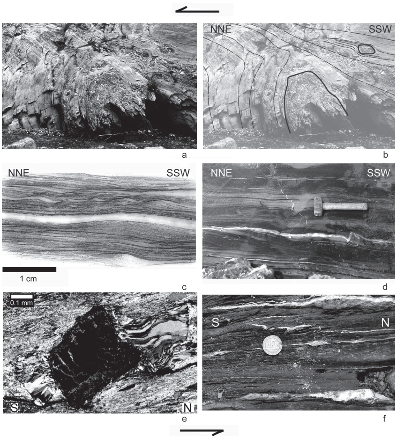
Fig. 5. Photographs of mesoscopic and microscopic sense of shear indicators (senses consistently sinistral in respect to photograph): a) & b) D2 Top-north shear sense in evaporites from the HF thrust, Gorges de Planlebon (see Fig. 7) c) Micrograph with shear bands and sigma clasts (bottom) in mylonitic Aalenian black shale (SBU), indicating top-NNE shear sense during D2 along the La Combe shear zone. d) Sheared veins in Aalenian black shales (SBU), indicating top-NNE shear sense during D2 along the Nant Brun shear zone. e) & f) top-N shear senses from syn-D2 SBF (preserved from D4 normal faulting in the Valbuche area); e) asymmetric fibrous growth in pyrite pressure fringes in silica-rich wild-flysch of the CNU; f) sheared veins and sigma clasts in Aalenian black shales of the SBU.
