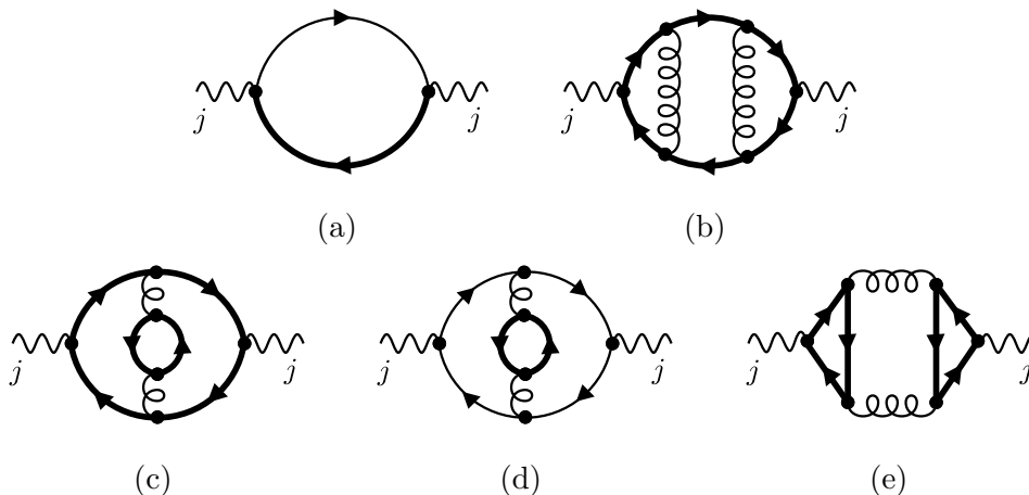
Figure 1. Sample diagrams contributing to the perturbative calculation of the VPF, i.e., the left-hand side of eq. (2.2). The currents are symbolized by wavy lines, gluons by spirals. We consider the case where n_l quarks are massless (thin straight lines), and n_h quarks are degenerate with mass m (thick straight lines). (a) One-loop contribution for non-diagonal currents; (b-e) sample three-loop diagrams for diagonal currents. In (d), the currents couple to massless quarks. (e) is a “singlet” diagram. All diagrams in this paper were produced with the help of FeynGame [25].
