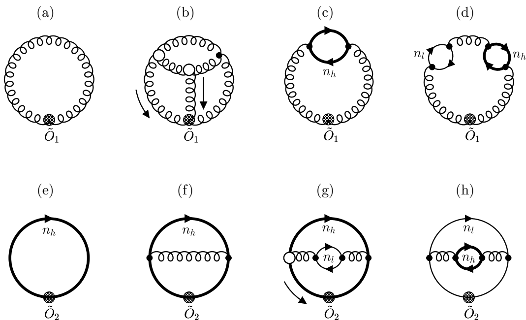
Figure 2. Sample diagrams contributing to \zeta_n^{(m)} ( m \in \{0, 2\} ) and \zeta_{n3} , for n = 1 (a-d) and n = 2 (e-h). The notation is the same as in figure 1; in addition, white circles denote flow-vertices, and lines with arrows next to them denote flow-lines (see ref. [65] for details). Diagrams (a) and (b) only contribute to \zeta_1^{(0)} .
