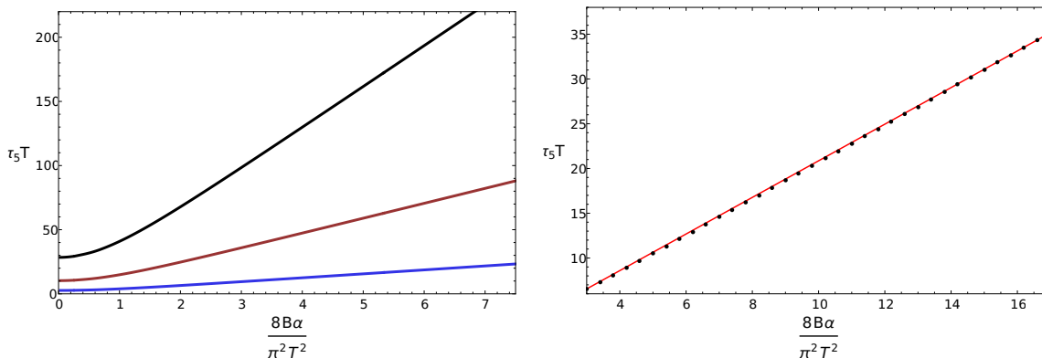
Figure 10. Left panel: axial charge relaxation time as a function of magnetic field for different values of the bulk mass m = 0.15 (Black), m = 0.25 (Red), m = 0.5 (Blue). Right panel: numerical data (dots) and linear fit (red) for \tau_5 at m = 0.5 and large magnetic field. The best fit in this region is \tau_5 T = 0.0979 + 0.5030 \frac{8B\alpha}{\pi^2 T^2 m^2} .
