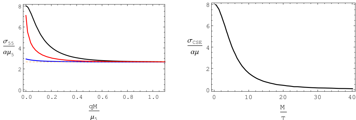
Figure 8. Left plot: \sigma_{55} as a function of the source M for 8B\alpha/\pi^2T^2 = 0.1 , \alpha = 1 , T/\mu_5 = 0.05 (blue), 0.075 (red), 0.1 (black). Note that T_c/\mu_5 \simeq 0.765 for this case. Dashed line \sigma_{55}/(\alpha\mu_5) = 8/3 . Right plot: \sigma_{\text{CSE}} as a function of M/T for B = 0 and \mu_5 = 0 while \mu \neq 0 . When M \rightarrow 0 , we have \sigma_{\text{CSE}} = 8\alpha\mu . For large M , \sigma_{\text{CSE}} \rightarrow 0 .
