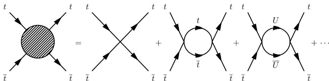
Figure 1. The \bar{t}t scattering amplitude in the J^P = 0^+ channel with the four-fermion kernel given by the terms in eq. (2.1).
