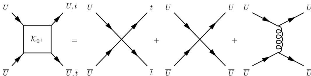
Figure 2. The kernel for scattering of \bar{U}U \rightarrow \bar{t}t and \bar{U}U \rightarrow \bar{U}U including ETC contact terms and one-TC-gluon exchange.
