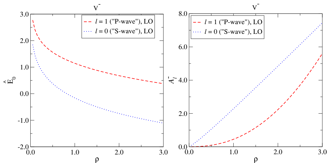
Figure 3. Left: the lowest “S-wave” and “P-wave” eigenvalues obtained with the LO potential V_{LO}^- (cf. eq. (6.31)). Right: the “amplitudes” corresponding to the lowest eigenmodes (cf. eq. (7.15)).
