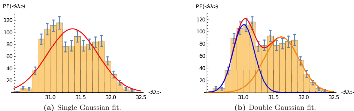
Figure 2. Double peak structure of the histogram of the chiral condensate at \kappa = 0.1665 and \beta = 5.6 from 1200 configurations. A single Gaussian does not fit our data, which are instead consistent with a sum of two Gaussian functions.
