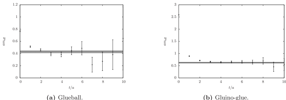
Figure 3. Mass plateau of the gluino-gluon and the 0^{++} glueball for \beta = 5.5 , \kappa = 0.1673 , on a 16^3 \times 32 lattice. The final value indicated by the gray line is obtained from a fit of the correlation function.
