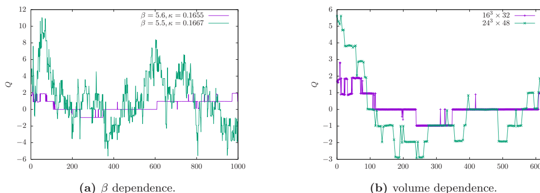
Figure 9. Left hand side: the history of the topological charge from simulations at \beta = 5.5 and \beta = 5.6 on a 16^3 \times 32 lattice. Right hand side: the history of the topological charge at \beta = 5.6 , \kappa = 0.1660 for two different volumes.
