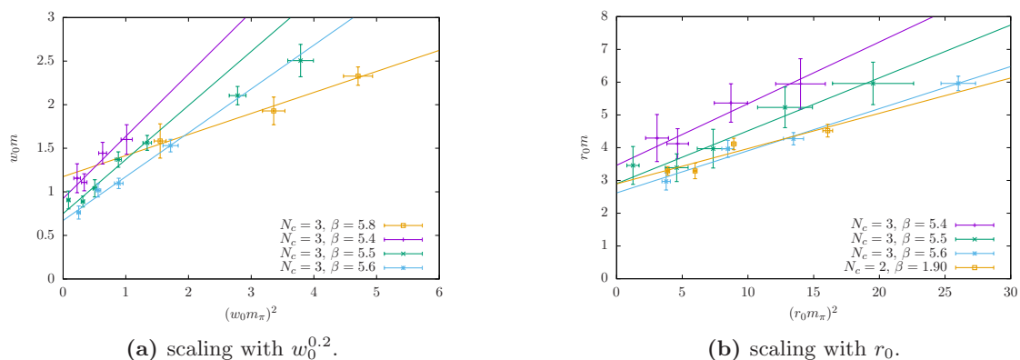
Figure 11. A comparison of the gluino-gluon mass in units of the Sommer scale r_0 and of w_0^{0.2} for different lattice spacings (corresponding to different \beta ) and SU(N_c) gauge groups as a function of the squared adjoint pion mass. The simulations of SU(3) SYM at \beta = 5.4, 5.5, 5.6 , and 5.8 have been done with a clover improved fermion action and a plain Wilson gauge action; the simulations of SU(2) SYM at \beta = 1.9 with a plain Wilson fermion action, one level of stout smearing, and a tree level Symanzik improved gauge action.
