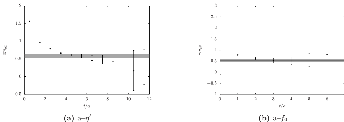
Figure 5. Mass plateau for the mesons a\text{-}\eta' and a\text{-}f_0 for \beta = 5.5 , \kappa = 0.1673 , on a 16^3 \times 32 lattice. The final value indicated by the gray line is obtained from a fit of the correlation function.
