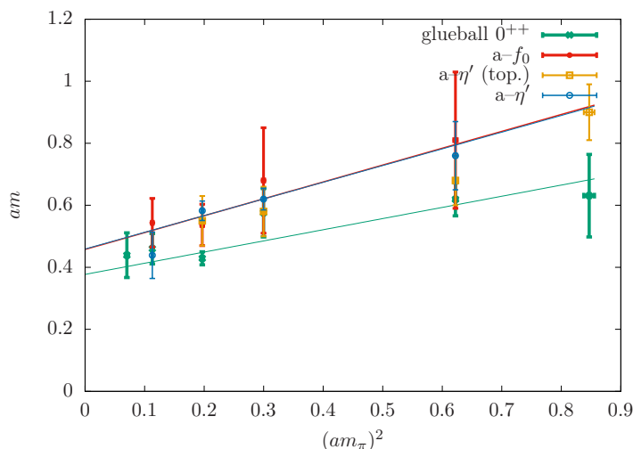
Figure 6. The masses of the different bosonic particles (singlet scalar and pseudoscalar mesons) in comparison to the glueball mass at \beta = 5.5 . a\text{-}\eta' (top.) indicates the pseudoscalar meson mass obtained from the topological charge density correlator.
