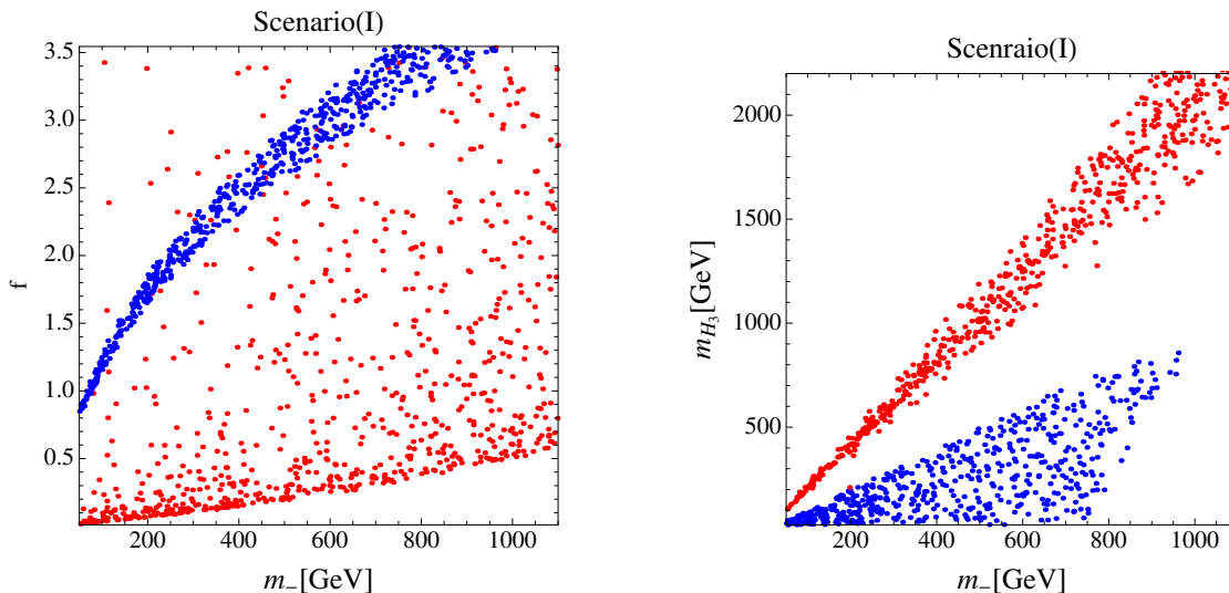
Figure 2. The parameter points providing required relic density of DM in scenario (I) where red and blue points correspond to the case of m_- + m_+ > m_{H_3} > m_- and m_- > m_{H_3} respectively.
