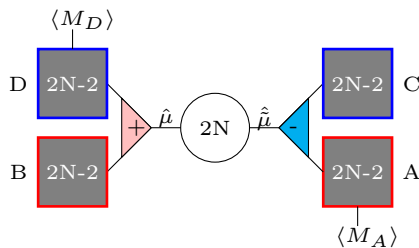
Figure 12: Crossing type dual \mathcal{U}_{c2}^{SO} of \text{SO}(2N) SQCD.
