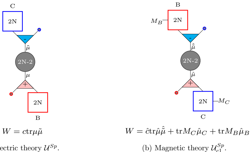
Figure 17: Intriligator-Pouliot duality.
