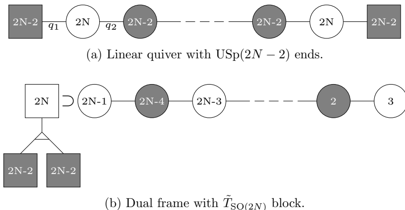
Figure 28: The linear quiver dual to \tilde{T}_{\text{SO}(2N)} coupled to a superconformal tail.
