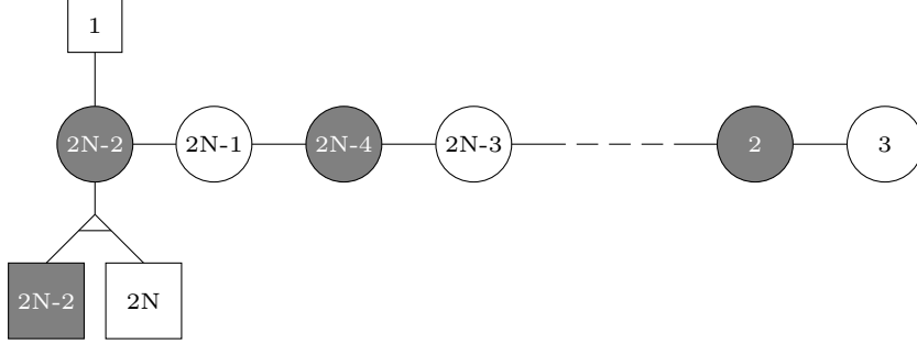
(b) Dual frame with \tilde{T}_{\mathrm{SO}(2N)} block.
