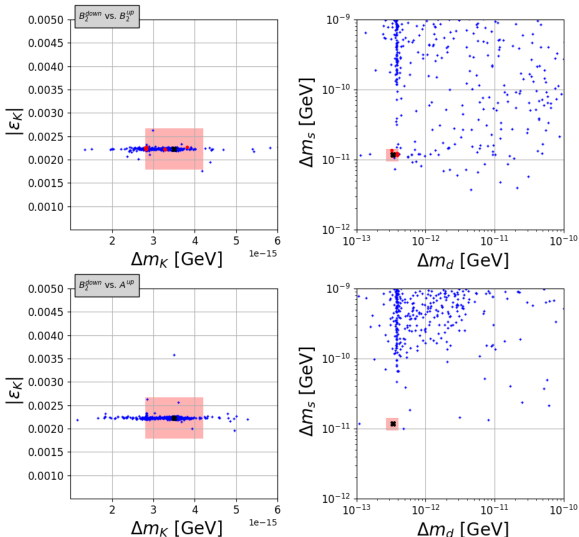
Figure 7. Meson sector predictions for (B_2, B_2) (upper) and (B_2, A) (lower) scenarios.
