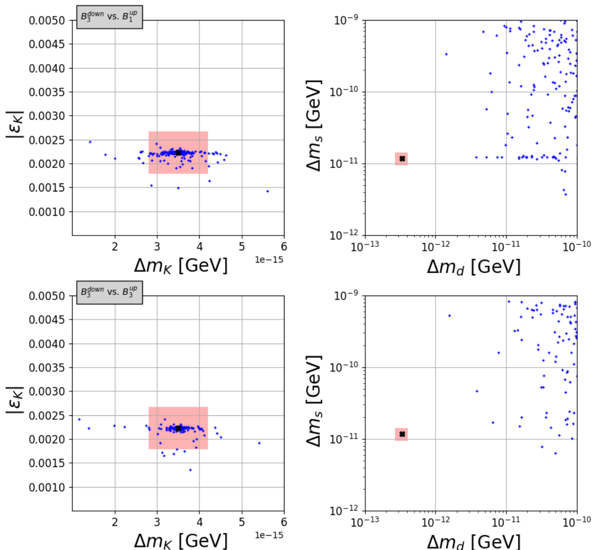
Figure 6. Meson sector predictions for (B_3, B_1) (upper) and (B_3, B_3) (lower) scenarios.
