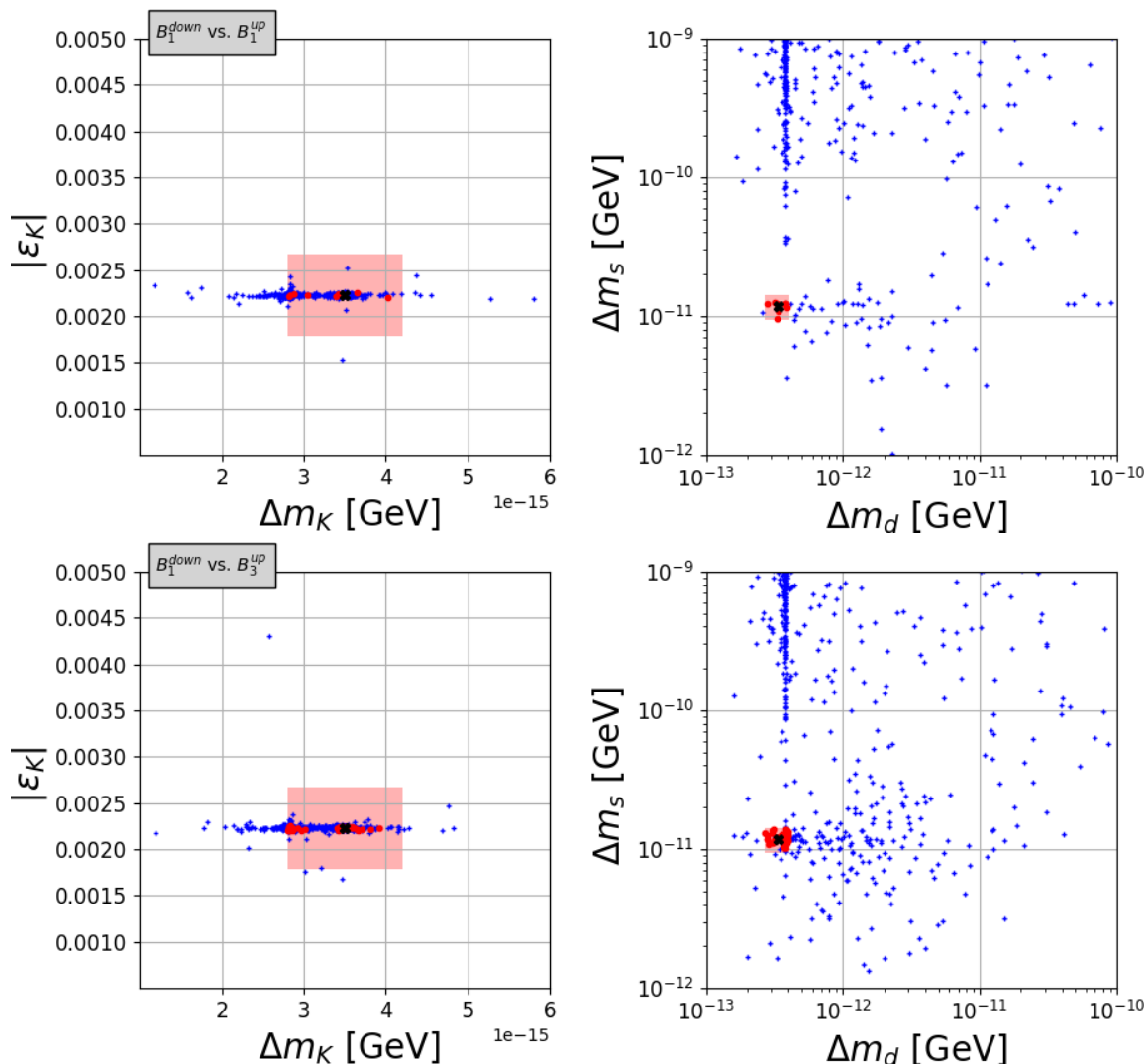
Figure 5. Meson sector predictions for (B_1, B_1) (upper) and (B_1, B_3) (lower) scenarios. The red dots indicate the points, which satisfy the K - and B -meson oscillations parameters within the chosen margins shown by pink rectangles.
