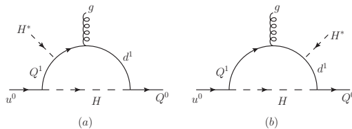
Figure 3. One-loop 1PI diagrams matching to chromomagnetic dipole operators.
