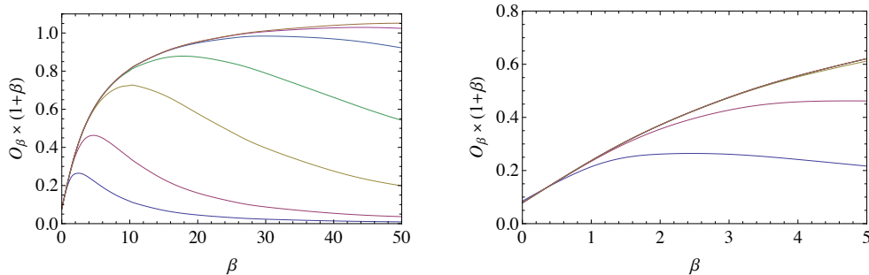
Figure 2. Bulk Higgs overlap function characterizing the size of the dipole contribution at one-loop. We have rescaled the 5D Yukawa by a factor \sqrt{1+\beta} in order to maintain the effective Yukawa finite in the large \beta limit. The various lines show the result of eq. (2.9) where the KK sums are performed up to 1,2,5,10,20,30,40 KK levels, from bottom to top. For values of \beta \gtrsim \mathcal{O}(10) (left plot) we find (1+\beta)\mathcal{O}_\beta \sim \mathcal{O}(1) , the overlap is suppressed for smaller values of \beta (right plot).
