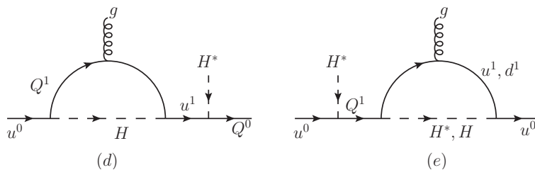
Figure 4. One-loop non-1PI diagrams matching to chromomagnetic dipole operators.
