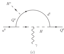
Figure 5. Additional one-loop 1PI diagram inducing magnetic dipole operators.
