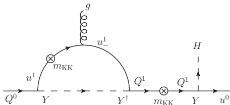
Figure 1. Leading one-loop diagram that contributes to the operator Q_8 from neutral Higgs exchange. Arrows denote the flow of charge through the diagram. Diagrams with a gluon radiated from the external quark legs are ignored as they contribute only to the gauge coupling renormalization.
