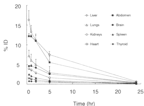
Fig. 3 Time-activity curves for various organs. Data were not corrected for decay and are expressed as percent injected radioactivity of [ ^{123}\text{I} ]5IA. Each point represents the mean \pm s.d. for all subjects.
