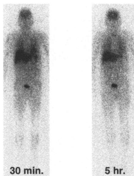
Fig. 2 Typical anterior whole-body images 30 min and 5 hr after the intravenous administration of [ ^{123}\text{I} ]5IA. Brain, lungs, liver and bladder were clearly visualized in both images.
