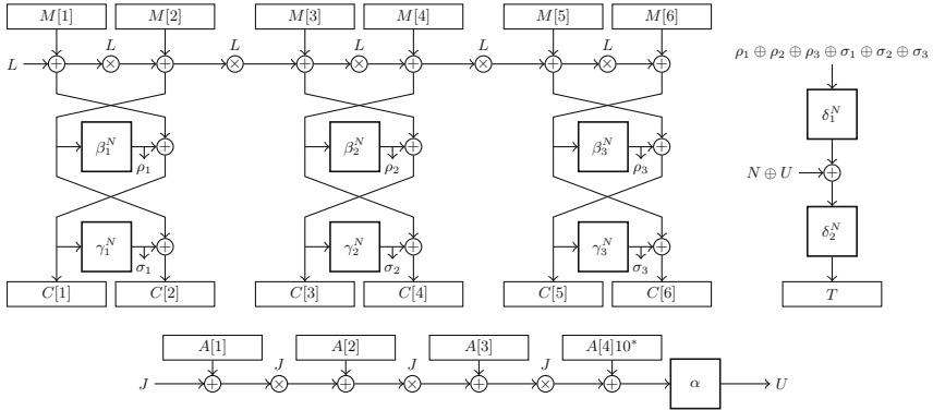
Fig. 4. Construction with independent URFs.
