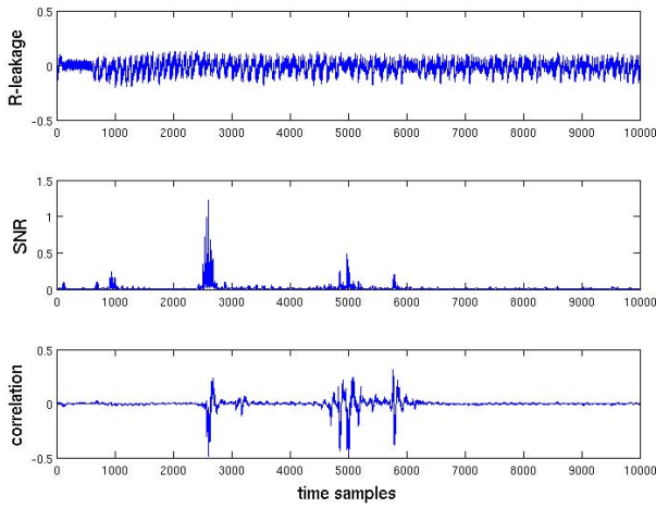
Fig. 8. Resistor-based measurements
