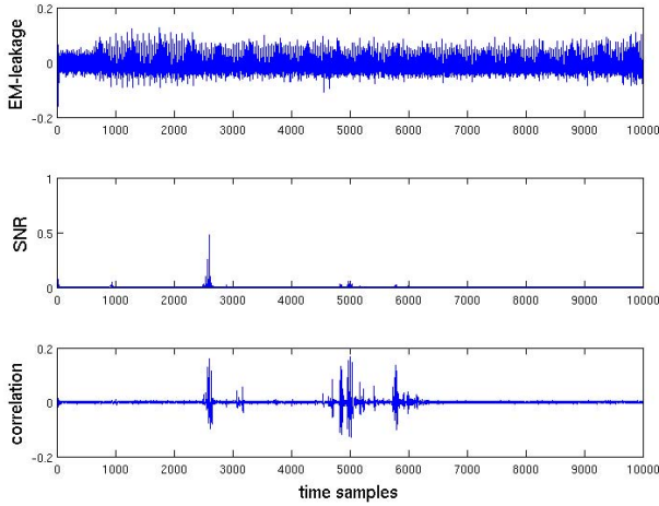
Fig. 10. Electromagnetic measurements
