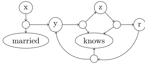
Fig. 1. Cyclic query
