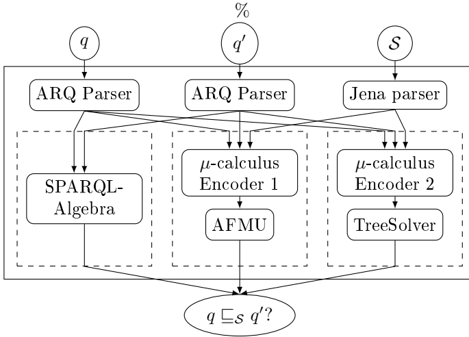
Fig. 2. Experimental setup for testing query containment. The tester (plain rectangle) parses queries and schemas and passes them to a solver wrapper (dashed rectangle).
