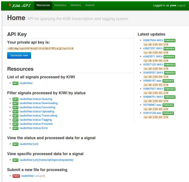
Fig. 2. The home page of KiWi API
