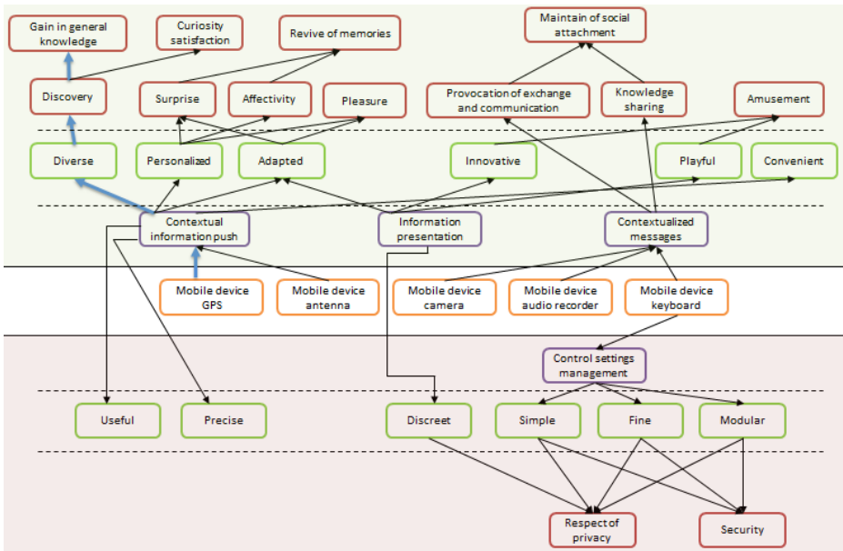
Fig. 2. The WM of Cocoon (partial) – The chain highlighted in blue can be read as follows: the contextual information push feature supported by the GPS of the mobile device presents the quality of being diverse (because serves the user with different types of information, personal and impersonal); this diversity enhances discovery of new things which results in a gain of general knowledge for the user.
