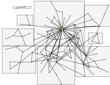
(b) BioJava, year 2006
