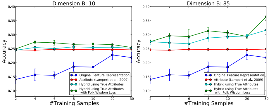
Fig. 4. Learning hybrid representations with and without folk wisdom loss using ground truth semantic attributes. Comparison with baselines methods using original feature representation (SURF features), and ground truth attribute representation [1] (mean and standard deviation over 5 runs). View across dimensions of the latent space \mathcal{B} .
