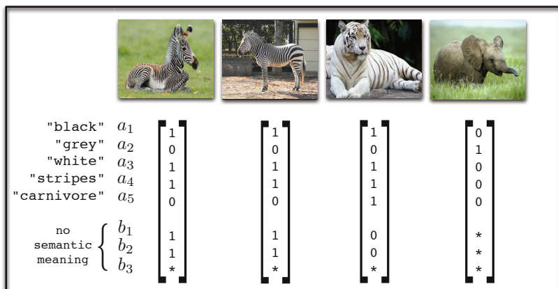
Fig. 1. Proposed hybrid representation: a fixed semantic ( a_1, \dots, a_5 ) part is augmented by a non-semantic ( b_1, \dots, b_3 ) part, where the latter is learned by enforcing a large margin separation criterion between classes. See Section 1 for a detailed description.
