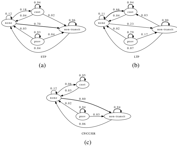
Fig. 7. Transition probabilities for links of STP, LTP, and CP/CC/ER monitors
