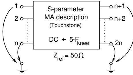
Fig. 7. Associated n-port model for an n-wire segment
