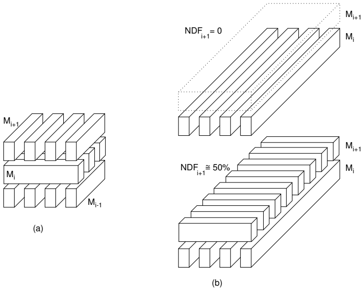
Fig. 5. (a) Orthogonal routing directions in adjacent metal layers. (b) NDF values of 0, respectively 50%.
