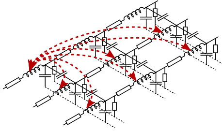
Fig. 1. Complexity of mutually-coupled inductances in distributed RLCG models
