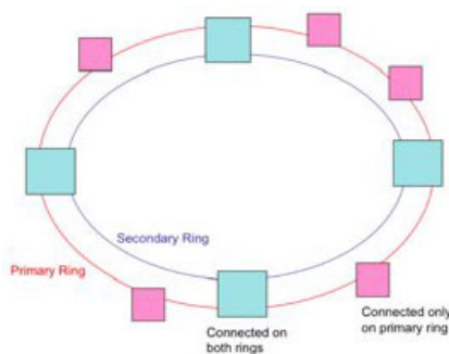
Fig. 1. Redundant double ring, implemented by frequency multiplex
