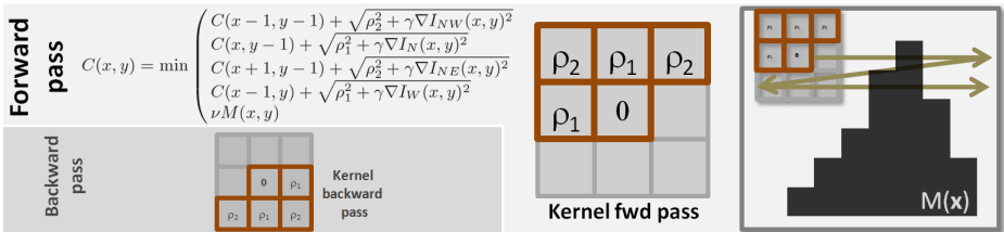
Fig. 12. Efficient geodesic distance transform. See appendix.
