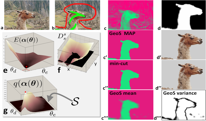
Fig. 4. GeoS v min-cut for interactive segmentation. (a) Input image. (b) user provided Fg and Bg strokes, (c) corresponding unaries (green for Fg, red for Bg and grey for uncertain). (d) ground truth segmentation (zoomed). (e) energy E(\alpha(\theta)) , with the computed minimum marked in red. (f) The distance D_s^s corresponding to the optimum \theta^* . (g) The proposal distribution q(\alpha(\theta)) . (c', d') Resulting GeoS MAP segmentation \alpha^* and corresponding Fg layer. (c'', d'') Min-cut segmentation on the same energy. (c''') GeoS mean segmentation \tilde{\alpha} , see text. Uncertain pixels are shown in grey. (d''') corresponding GeoS variance (dark for high variance).
