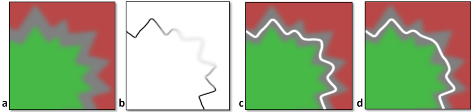
Fig. 3. Filter behaviour in the presence of weak unaries. (a) Input unaries (green for F_g and red for B_g ), with large uncertain areas (in grey). (b) Magnitude of gradient of input image. (c) Computed segmentation boundary (white curve) for a small value of \theta_d = \theta_e . (d) As in (c) but for large \theta . Larger values of \theta yield smoother segmentation boundaries in the presence of weak edges and/or weak unaries. In contrast, strong gradients “lock” the segmentation in place.
