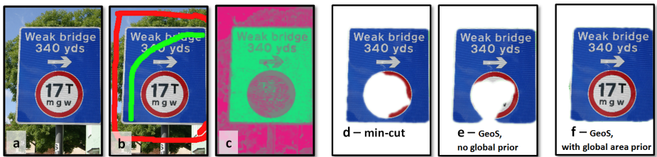
Fig. 9. Exploiting global constraints. (a) Original test image; (b) user provided F_g and B_g strokes; (c) corresponding unaries; (d) min-cut segmentation with \kappa = 0 ; The circular traffic sign is missed out. (e) GeoS segmentation on same energy as in (d); (f) GeoS segmentation on energy with global constraint G = |Area_{F_g}/Area - 0.7| .
