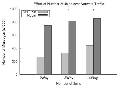
Fig. 3. Effect of Number of Joins
