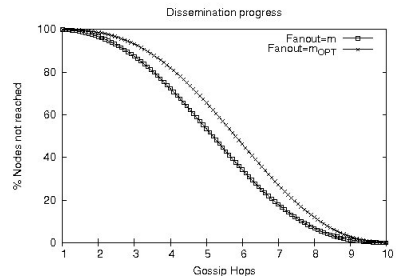
Fig. 4. Dissemination progress
