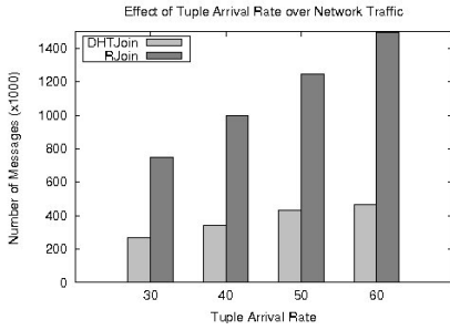
Fig. 1. Effect of Tuples Arrival Rate
