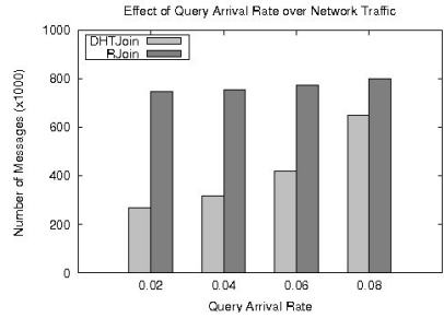
Fig. 2. Effect of Query Arrival Rate
