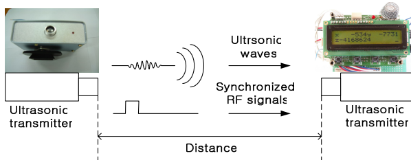
Fig. 2. Ultrasonic distance measurement system
