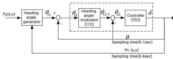
Fig. 7. Block diagram of feedback loop by using heading angle modulator
