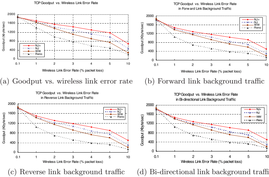
Fig. 5. TCP NJ+ goodput performance
