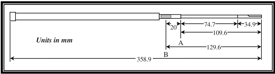
Fig. 1. Assembled Device Dimensions
