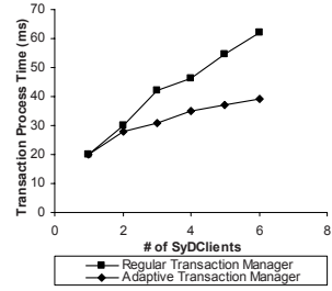
Fig. 7. Transaction Quality.
