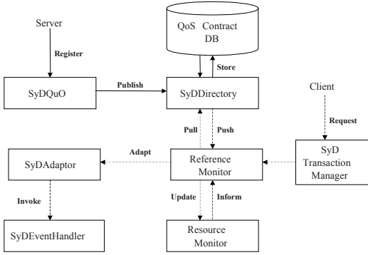
Fig. 6. QoS-aware Transaction.
