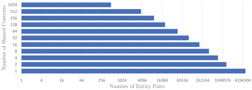
Fig. 12. Number of contexts for an entity pair
