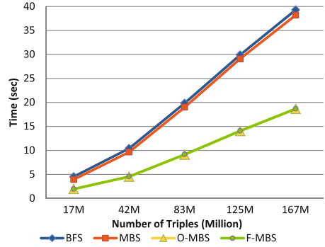
Fig. 7. Execution time vs data size (Jena)
