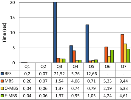
Fig. 6. Execution time (Virtuoso)
