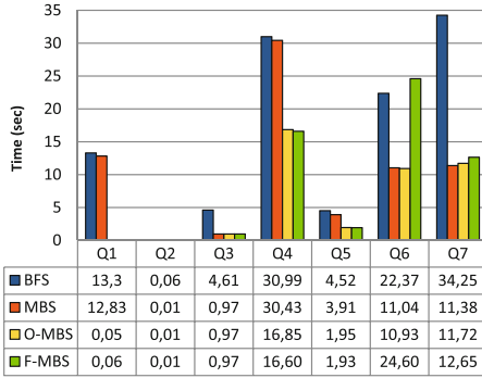
Fig. 4. Execution time (Jena)
