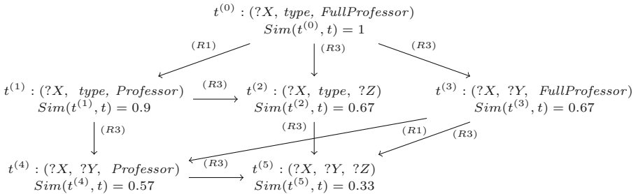
Fig. 2. Relaxation of a triple pattern
