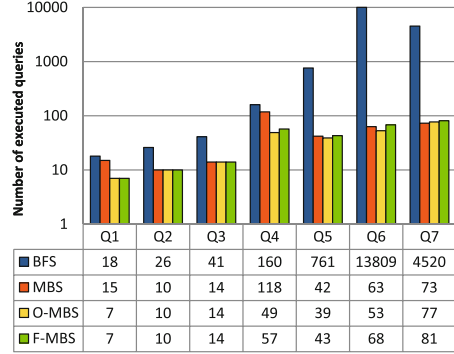
Fig. 5. # Executed queries (log scale)
