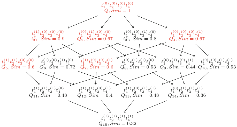
Fig. 3. Query relaxation graph
