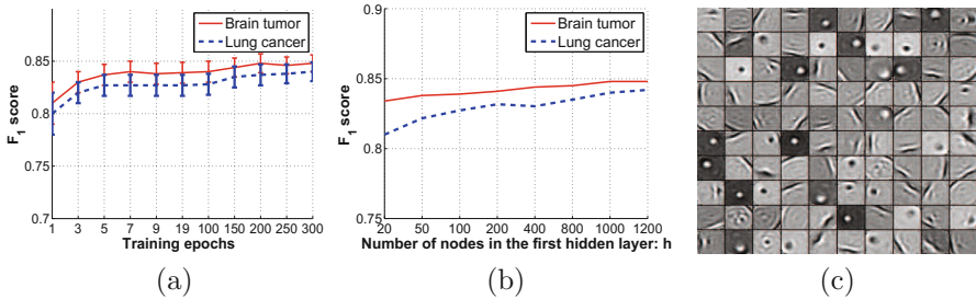
Fig. 4. (a) F_1 score as a function of the number of training epochs. (b) F_1 score as a function of the model complexity. (c) A set of learned feature maps in the first hidden layer.
