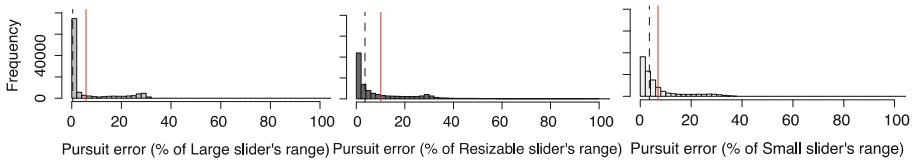
Fig. 7. Distribution of the pursuit error for each device condition (large, resizable and small). Dashed lines show the medians and red lines show the means (Color figure online).
