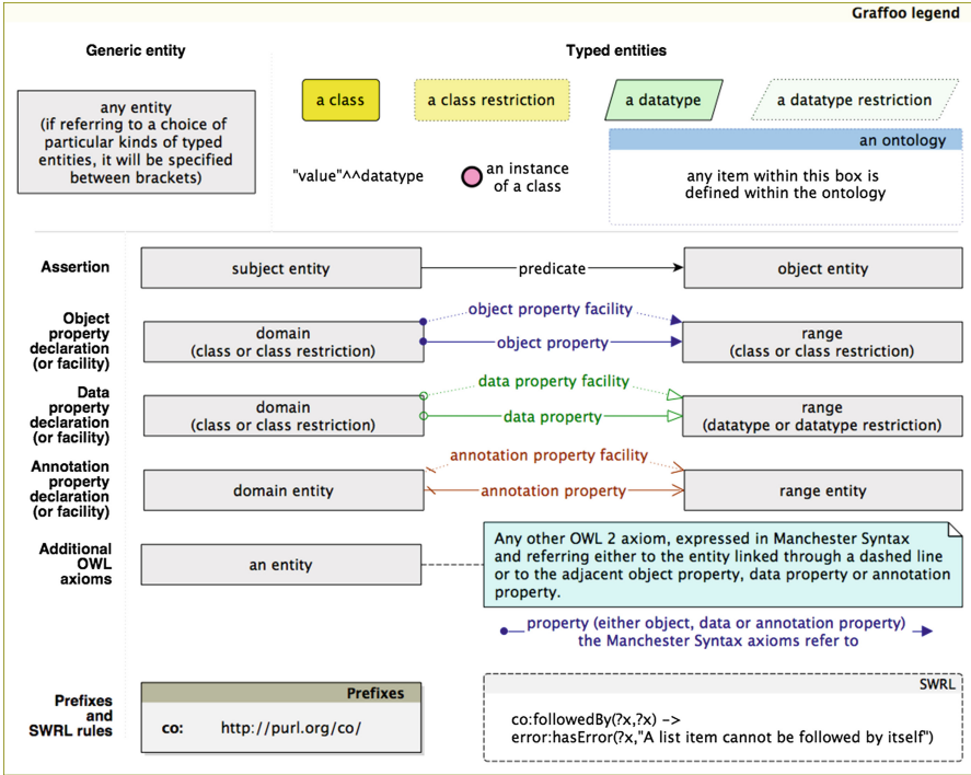
Fig. 1. The full set of graphical elements of Grafoo.
