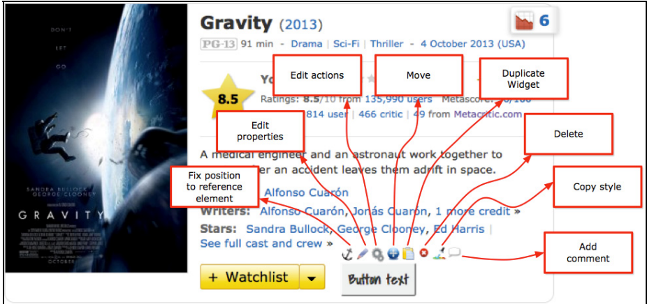
Fig. 8. Widget contextual menu
