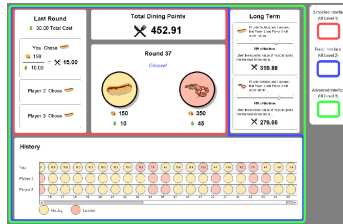
Fig. 3. The second Diner’s Dilemma study with three UI levels
