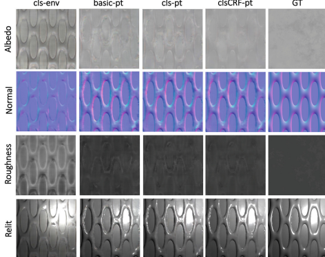
Fig. 6. Qualitative comparison of BRDF reconstruction results of different variants of our network. The notation is the same as Table 3 and -env represents environment illumination.
