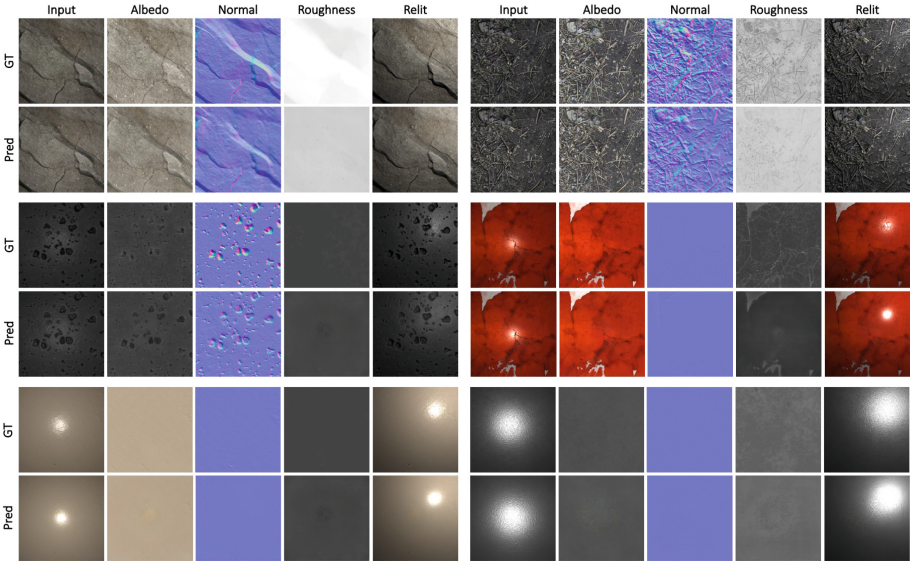
Fig. 4. BRDF reconstruction results from our full method (clsCRF-pt in Table 3) on the test set. We compare the ground truth parameters with our reconstructions as well as renderings of these parameters under novel lighting. The accuracy of our renderings indicates the accuracy of our method.
