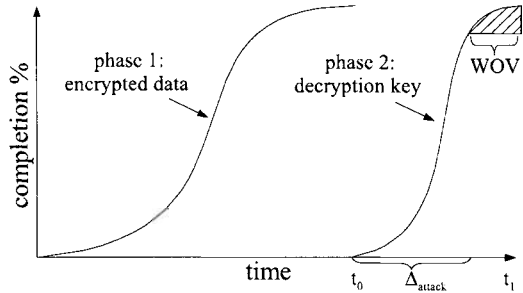
Fig. 2. Two-Phase dissemination
