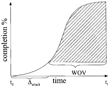
Fig. 1. Cleartext dissemination
