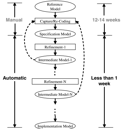
Figure 1. Motivation: Design time of MP3 decoder in a refinement-based design flow.
