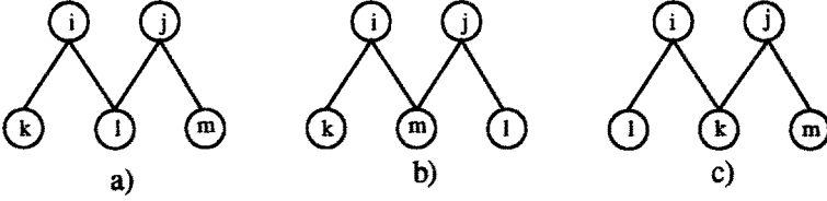
Fig. 2. Dome paths
