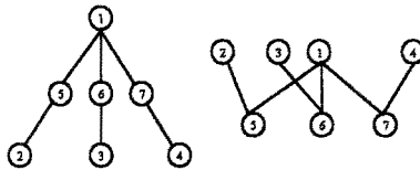
Fig. 1. 3-claw graph
