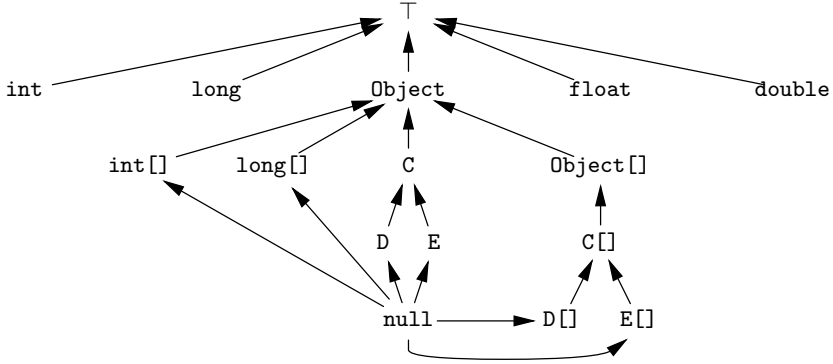
Fig. 3. Type expressions used by the verifier, with their subtyping relation. C, D, E are user-defined classes, with D and E extending C. Not all types are shown.
