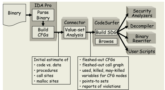
Fig. 1. Organization of CodeSurfer/x86
