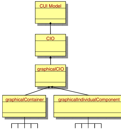
Fig. 6. Decomposition of a CUI model into concepts
