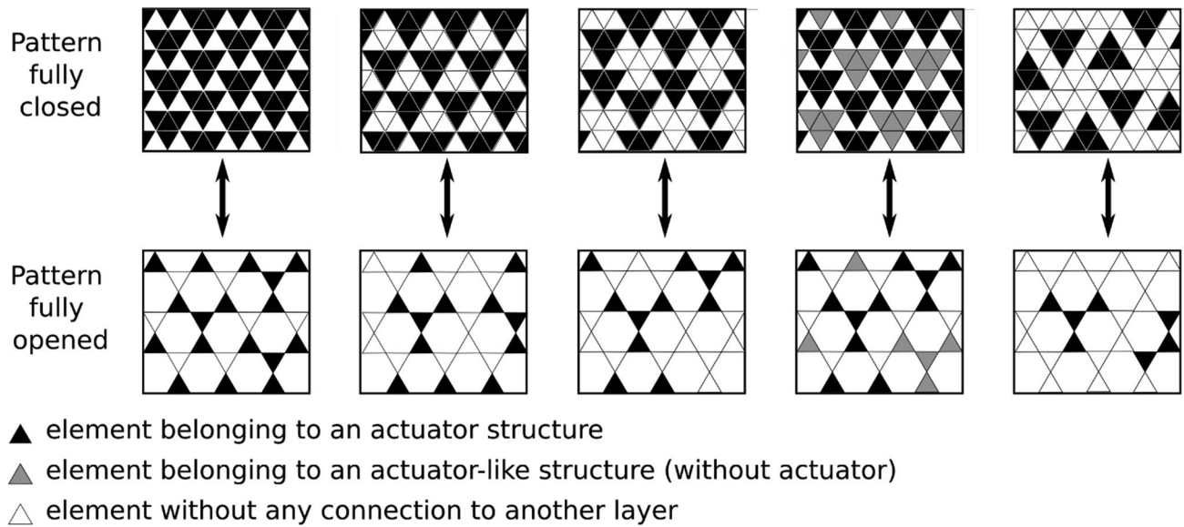
Figure 9 Schematic representation of controllable auxetic structures with multiple DOFs in closed and open configuration. Here, black triangles represent elements which are attached to an
