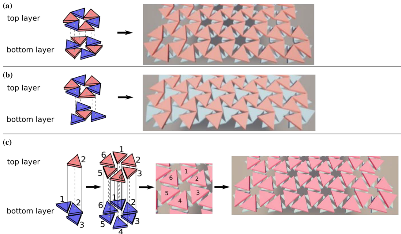
Figure 5 Basic variants of kagome-based two-layered structures. In variant a , the top layer and the bottom layer are mirrored, and all elements of the top have interlayer connections to the bottom layer
